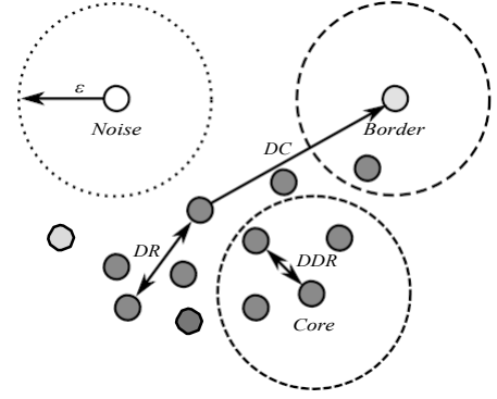
Figure 1: DBSCAN clustering with minPoints = 4
